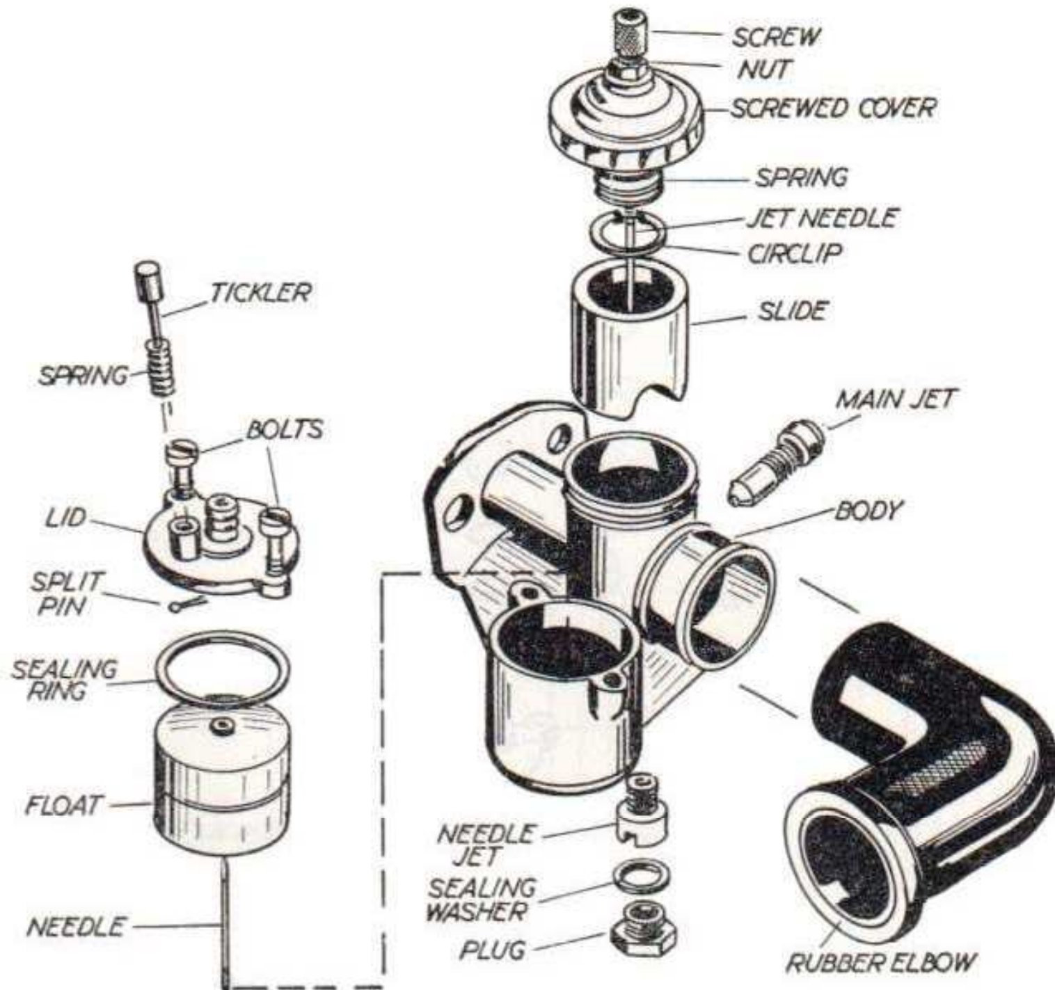
FIG. 40. AN EXPLODED VIEW OF THE CARBURETOR USED ON THE TWO-SPEED MODELS SHOWING ALL PARTS
