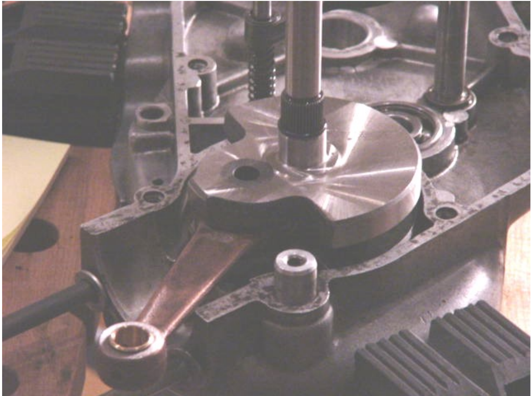
The crankshaft is inserted
